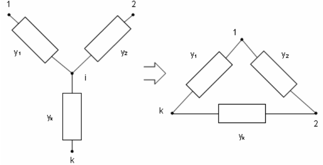
Fig. 3. A work node of RLC circuit. Addition of a conductance between node 1 and nodes next to i -th.
